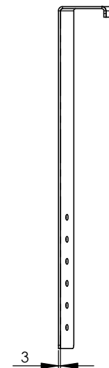
Part: 9493-12 Drum retainer pressing L Material: Mild steel
