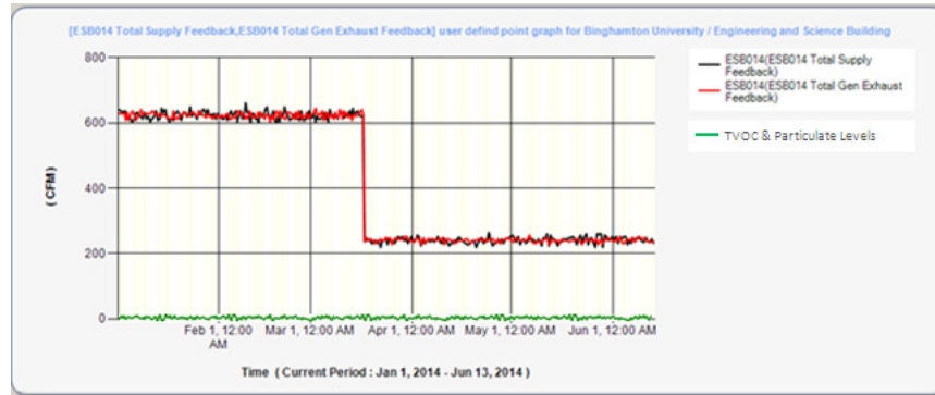
Figure 1. CFMs were reset in mid March 2014. Room ESB014 base: 624 CFM, 10 ACH; post OptiNet targets achieved: 238 CFM, 4 ACH.
