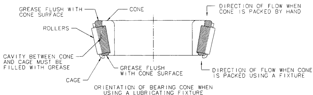
Figure 313 - Packing Bearing Cones
