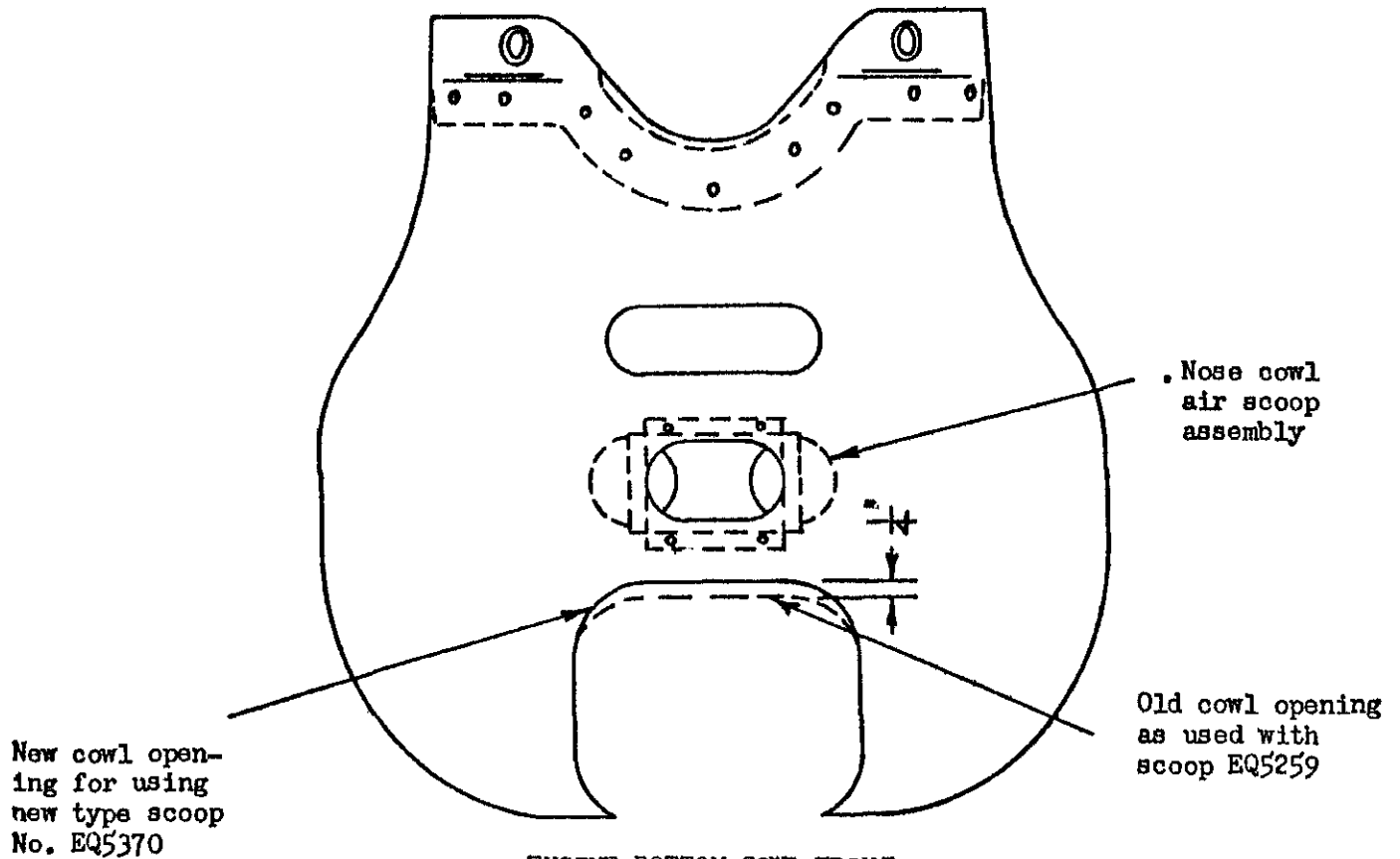
ENGINE BOTTOM COWL FRONT
