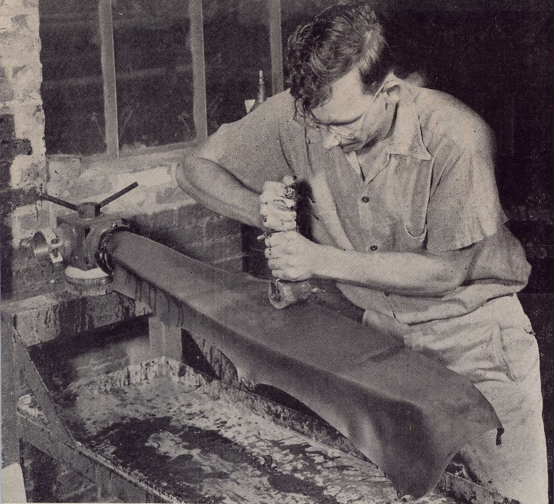
5—The plastic sheet is hand rolled to the blade for the purpose of eradicating irregularities and achieving bond
