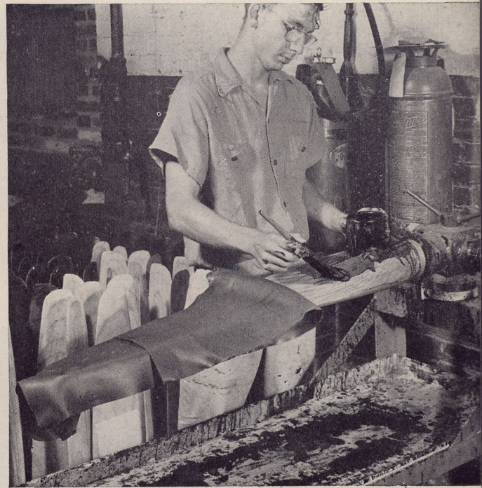
3—(Left) After suspension for an hour in a softening solution the nitrate sheet is ready for application to the blade. 4—(Right) Plastic cement is first applied to top side of blade and to half of plastic sheet
