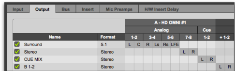
Standard 5.1 format (film) output paths
