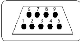
D-Sub 9-Pin Female
