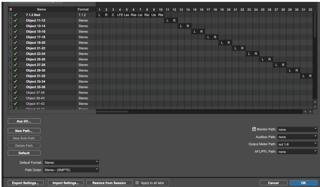
I/O Setup, Output page configured for playback to a Dolby Atmos Renderer
