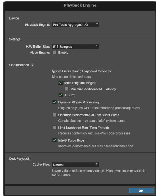
Playback Engine using Pro Tools Aggregate I/O (Mac)
