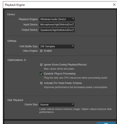
Playback Engine using Windows Audio Device
