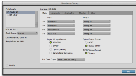
Hardware Setup for HD OMNI, Main page
