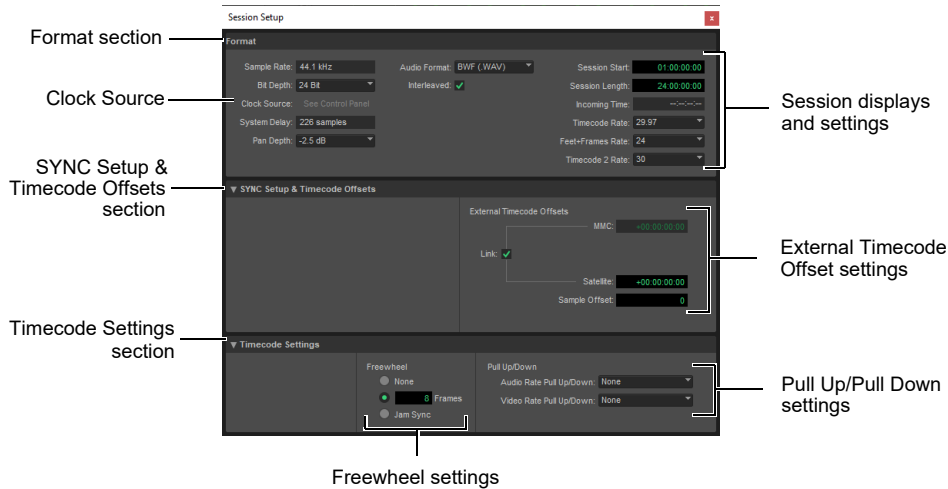
Session Setup window with no synchronization peripheral
